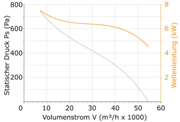
DHPX/SEC-100-4T-10
