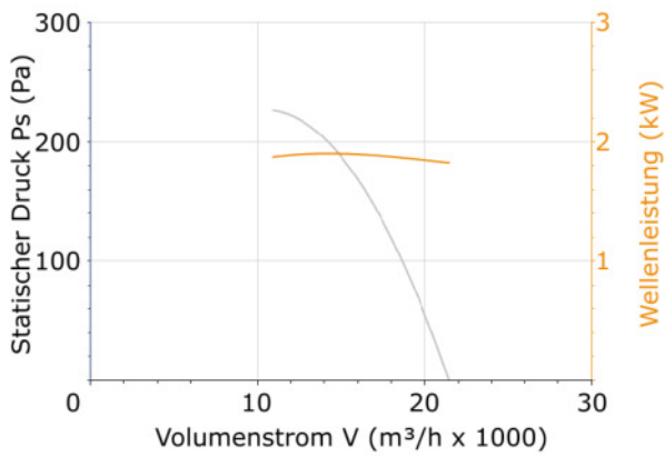
DHPX/SEC-63-4T-3
