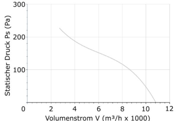
DHPX-50-4T-1
