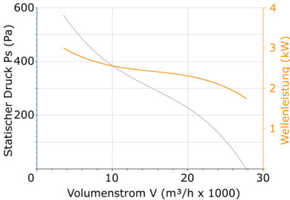
DHPX/SEC-80-4T-4
