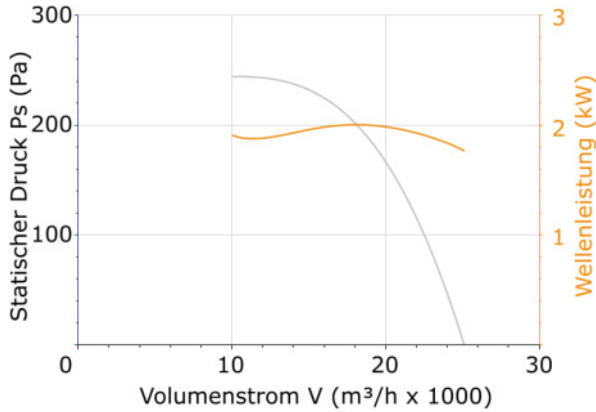
DHPX/SEC-71-4T-3
