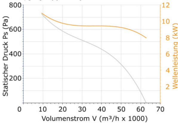
DHPX/SEC-100-4T-15
