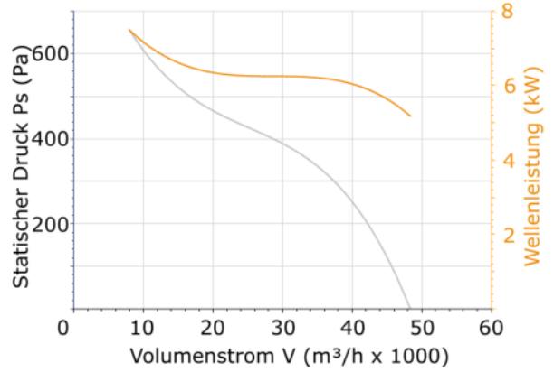
DHPX/SEC-90-4T-10
