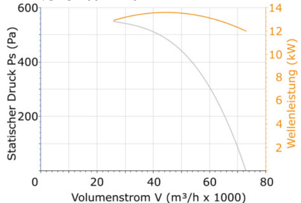
DHPX/SEC-100-4T-20
