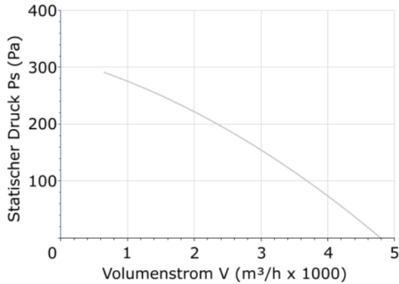
DHPX-35-2T
