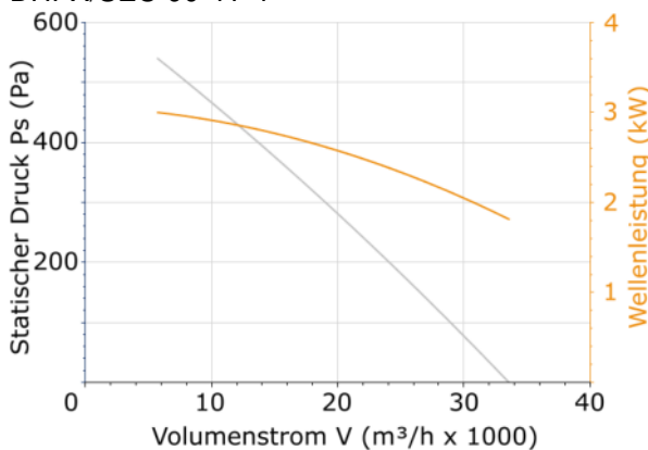
DHPX/SEC-90-4T-4
