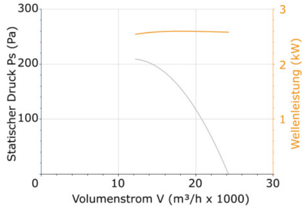
DHPX/SEC-4T-4
