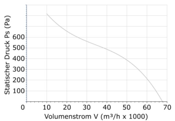
DHPX-100-4T-15
