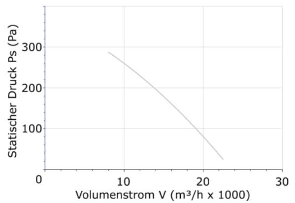
DHPX-71-4T-2
