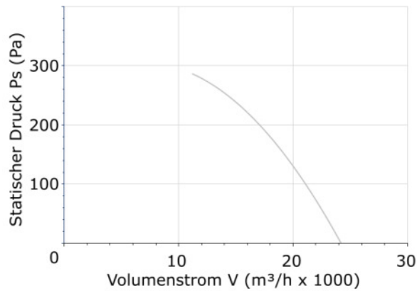
DHPX-71-4T-3
