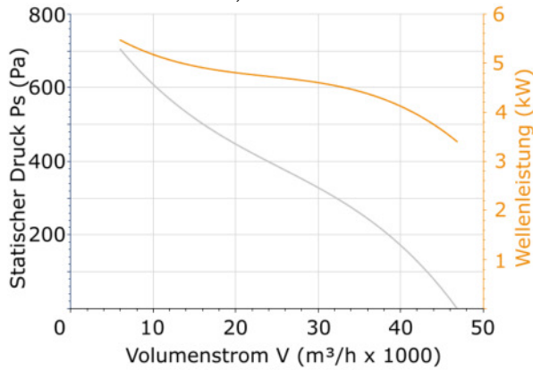
DHPX/SEC-100-4T-7,5
