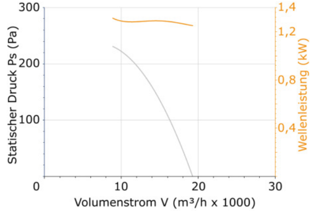
DHPX/SEC-63-4T-2
