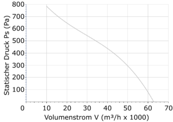
DHPX-100-4T-10
