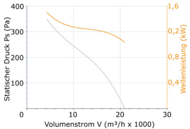
DHPX/SEC-71-4T-2
